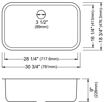
MODEL: E-340 Stainless Steel Large Single Bowl Seamless Kitchen Sink
