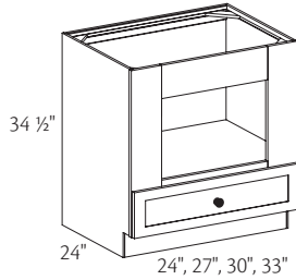
Cut-out Single (COS) for Base Microwave Cabinet Trimmable
