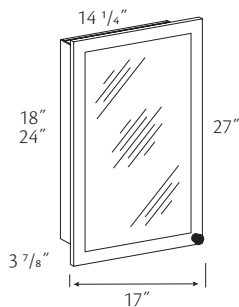
Rough-in dimensions
