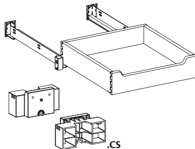
Deluxe Dovetail Roll-out Tray Field Installation Chart
