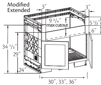
Cut out dimensions
