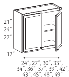
Shown with center stile
