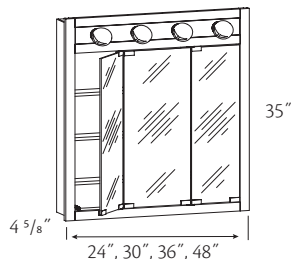
Rough-in dimensions
